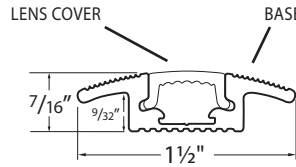
CC & CW Wire Way Combo - Base & Lens WW-CC-BK-8 Carpet to Carpet Base and Cover 8' - Black WW-CC-GY-8 Carpet to Carpet Base and Cover 8' - Gray WW-CW-BK-8 Carpet to Wall Base and Cover 8' - Black WW-CW-GY-8 Carpet to Wall Base and Cover 8' - Gray
